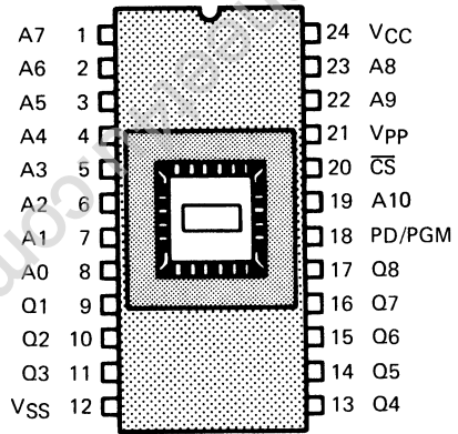
24-PIN CERPAC DUAL-IN-LINE PACKAGE (TOP VIEW)
